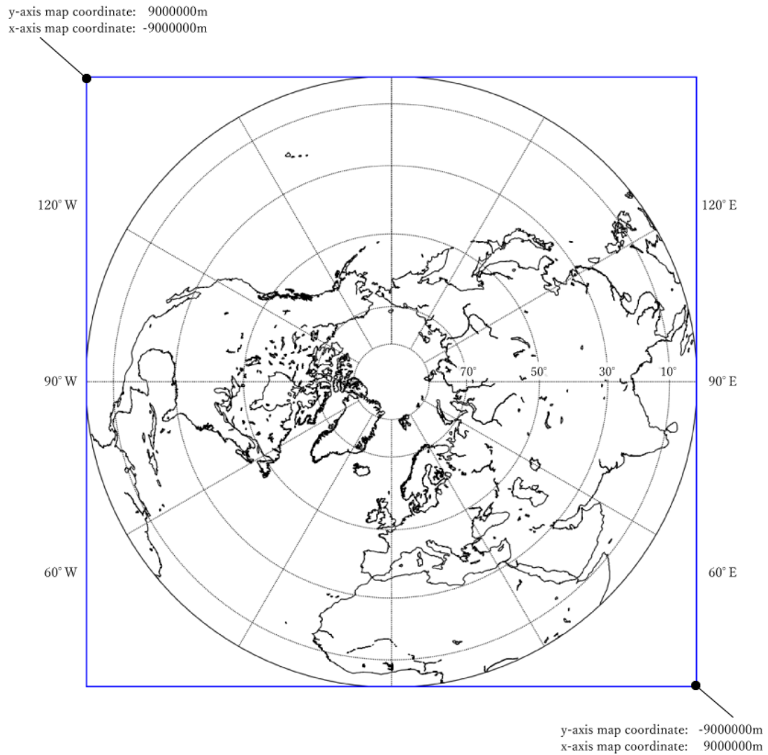
Figure 3.4-6 EASE-Grid 2.0 Projection Definition (Northern Hemisphere, Lambert Azimuthal)
