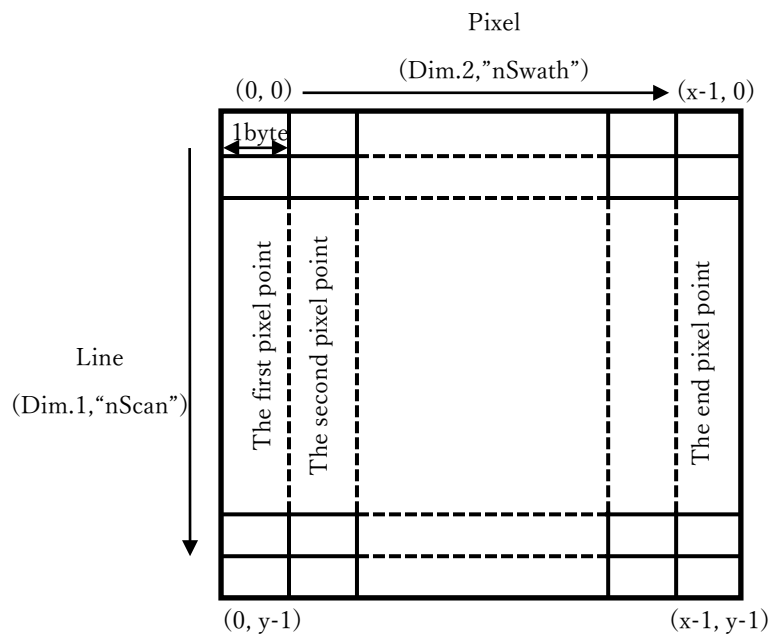
Figure 3.3-3 Structure of Data<n>_Quality (Daily/Monthly)
